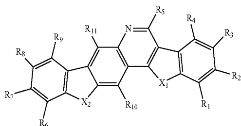
Formula 2D
