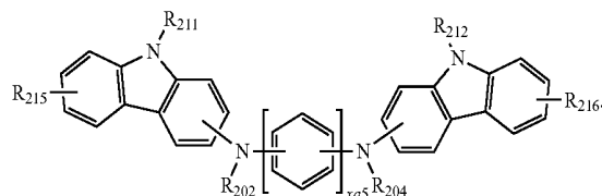
&lt;Formula 202A&gt;
