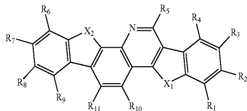
Formula 2B
