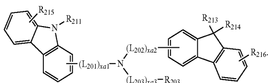
&lt;Formula 201A&gt;
