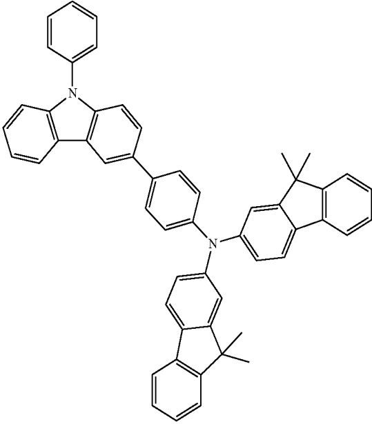
HT9
