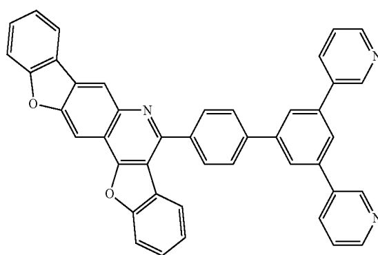
compound 64
