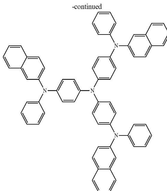
2-TNATA
