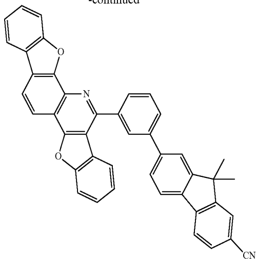
compound 20
