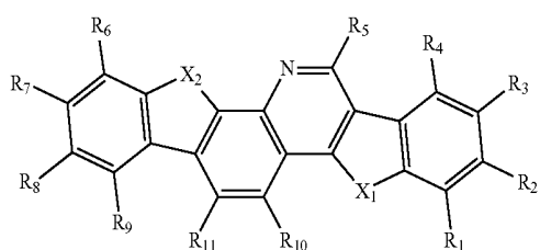
Formula 2A
