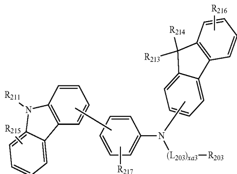
&lt;Formula 201A(1)&gt;
