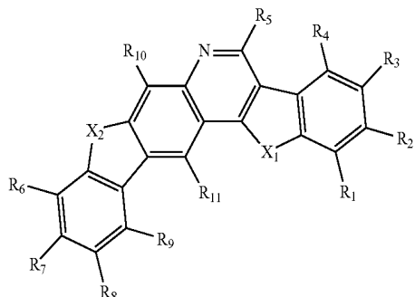
Formula 2D
