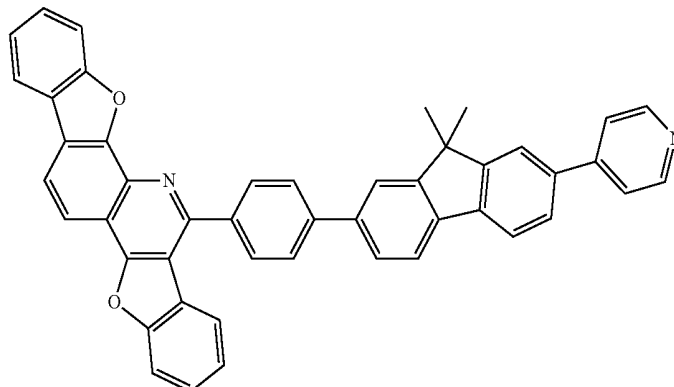
compound 23
